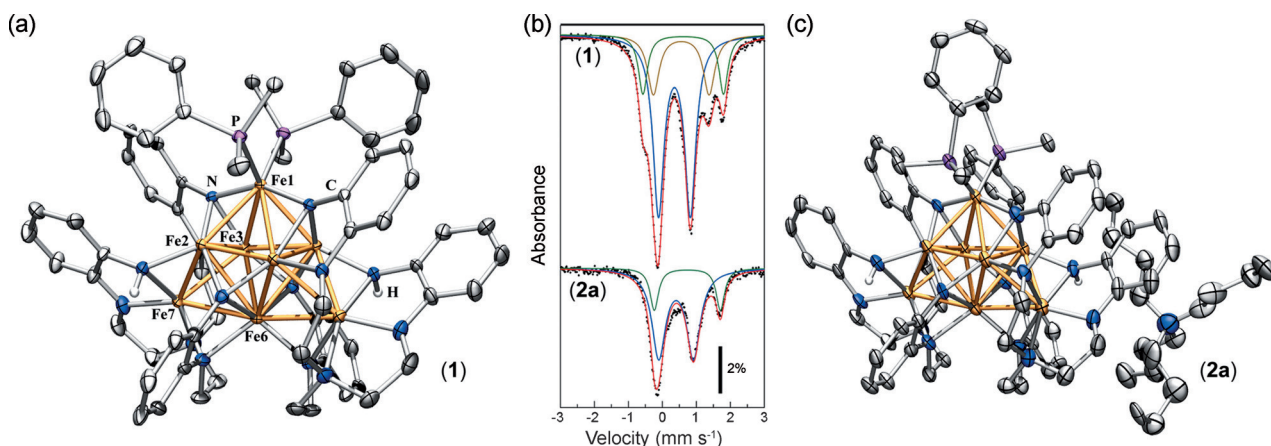
Figure 1. Molecular crystal structures of a) [(^{\text{tren}}\text{L})_2\text{Fe}_8(\text{PMe}_2\text{Ph})_2] ( 1 ) and c) [\text{Bu}_4\text{N}][(^{\text{tren}}\text{L})_2\text{Fe}_8(\text{PMe}_2\text{Ph})_2] ( 2a ) with thermal ellipsoids set at 50% probability; hydrogen atoms and solvent molecules omitted for clarity. Atom colors: Fe = orange, C = gray, N = blue, H = white, P = magenta. b) Zero-field ^{57}\text{Fe} Mössbauer spectra for 1 (top) and 2a (bottom). The black-dotted trace shows the experimentally obtained data and the red trace is an average of the model fittings. Component parameters for the model fittings of the spectrum of 1 ( \delta , |\Delta E_Q| ; measured in \text{mm s}^{-1} ): 0.35, 0.94 (60%, blue trace); 0.55, 1.64 (20%, brown trace); 0.61, 2.37 (20%, green trace). Parameters for the model fittings of 2a ( \delta , |\Delta E_Q| ; \text{mm s}^{-1} ): 0.40, 1.02 (67%, blue trace); 0.73, 1.95 (33%, green trace).
