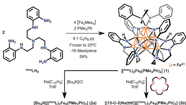
Scheme 1. Synthesis of [(^{\text{tren}}\text{L})_2\text{Fe}_8(\text{PMe}_2\text{Ph})_2] and its anion. Py = pyridine.
